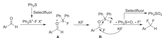
Scheme 4. The plausible reaction mechanism.
