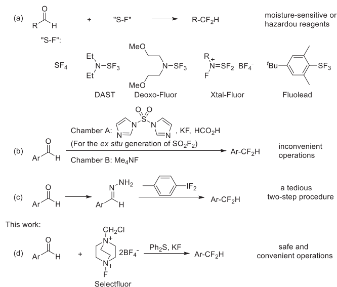
Scheme 1. Deoxydifluorination of aldehydes.
