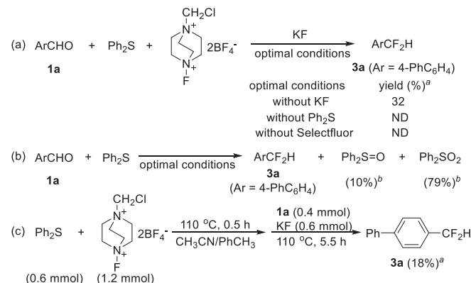
Scheme 3. Experimental evidence. a The yield was determined by 19 F NMR spectroscopy; b Isolated yields were calculated based on substrate 1a .
