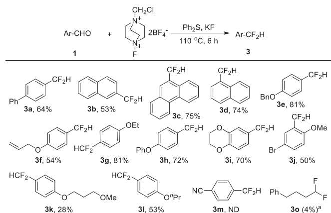
Scheme 2. Deoxydifluorination of aldehydes. Reaction conditions: substrate 1 (0.4 mmol), Ph 2 S (0.6 mmol), Selectfluor (1.2 mmol) and KF (0.6 mmol) in CH 3 CN/PhCH 3 (1 mL/1 mL) at 110 °C for 6 h under a N 2 atmosphere. a The yield of 3o was determined by 19 F NMR spectroscopy.
