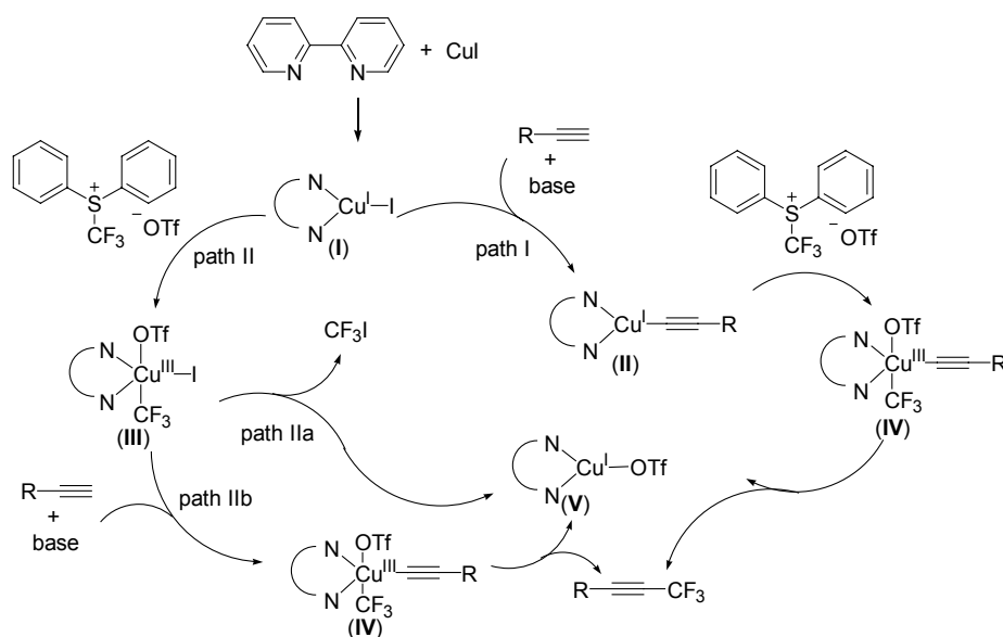
Scheme 1 Proposed mechanism for the trifluoromethylation of terminal alkynes
