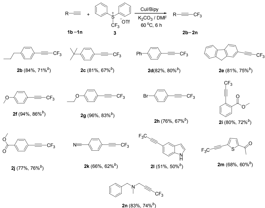
Figure 1 CuI-mediated trifluoromethylation of terminal alkynes (the molar ratio of 1b–1n : 3 : CuI : Bipy : \text{K}_2\text{CO}_3 was 1 : 2 : 1 : 1. The yield was determined by ^{19}\text{F} NMR. b Isolated yield).
