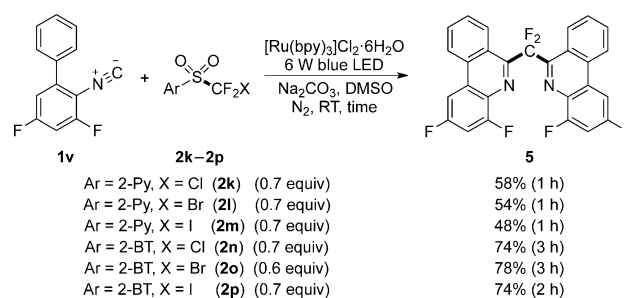
Scheme 2. Fluoroalkylation with halodifluoromethyl sulfones. 2-BT = 2-benzo[d]thiazolyl.
