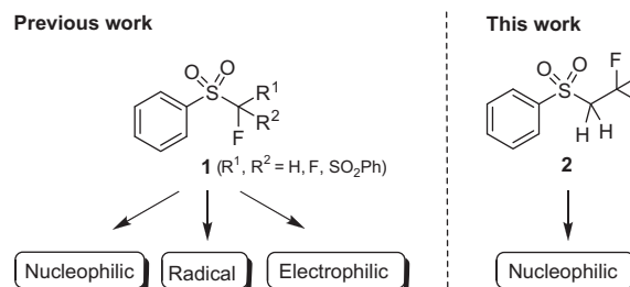
Scheme 1. Different (phenylsulfonyl)fluoroalkylations.
